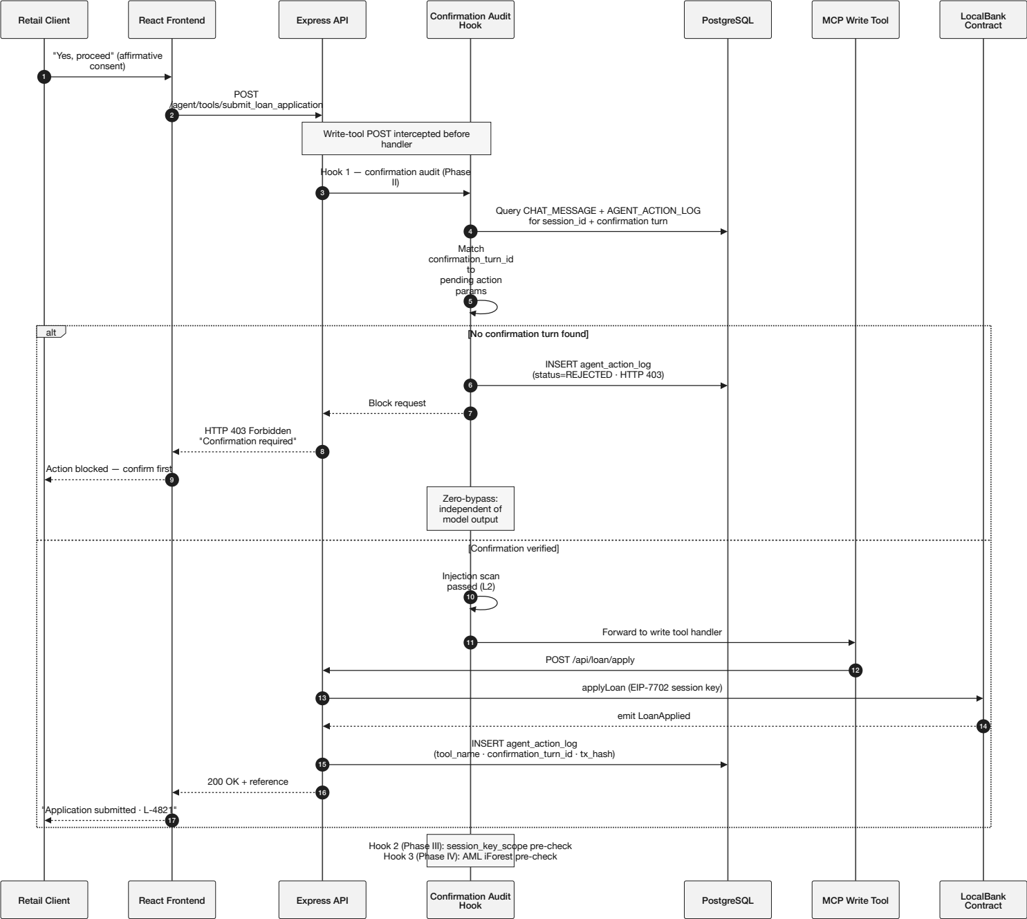
Sequence Diagram — Agent Confirmation Gate Middleware (HTTP 403)
